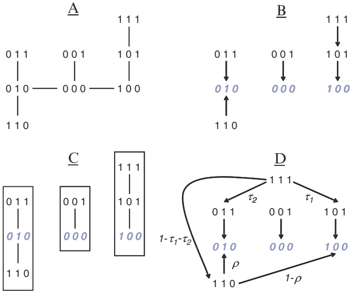
Fig. 3 (a) Cladogram of 3-SNP haplotypes. (b) Assignment of haplotypes to closest cluster base (shown in grey shadow ). (c) Resulting three haplotype clusters from (b). (d) Haplotype clustering using a probabilistic algorithm
